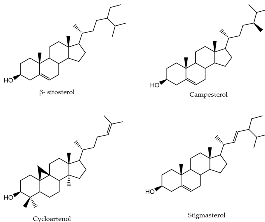
Figure 5. Chemical structures of detected phytosterols in espresso coffee.
