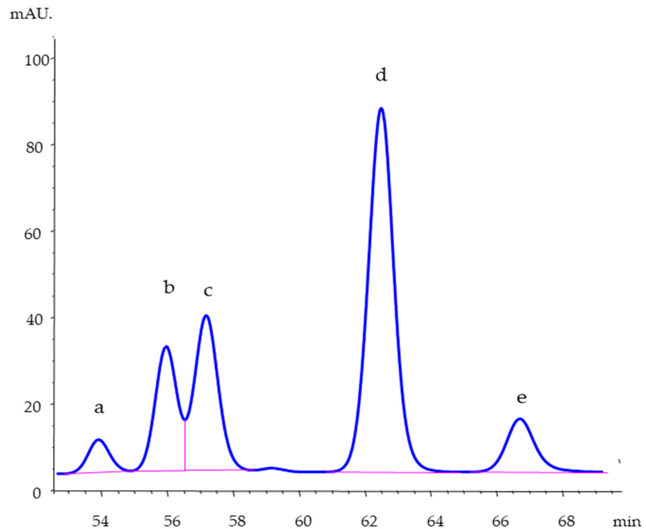
Figure 4. Chromatogram of phytosterols in espresso coffee from Costa Rica coffee-origin (sample No. 4), a for cycloartenol, b for campesterol, c for stigmasterol, d for \beta -sitosterol, and e for hexacosanol (internal standard).
