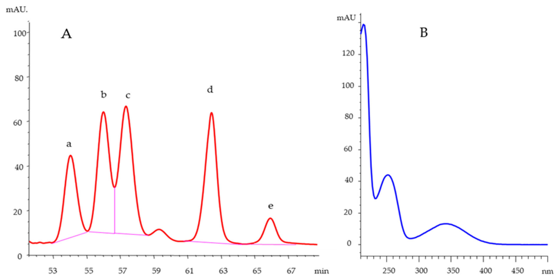
Figure 3. (A) Chromatogram of phytosterols standard solution at 100 mg/L: a for cycloartenol, b for campesterol, c for stigmasterol, d for \beta -sitosterol, and e for hexacosanol (internal standard); (B) UV spectrum of derivatized phytosterols.
