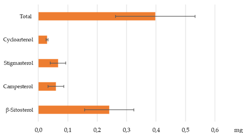
Figure 6. Mean levels of phyosterols (mg) in one cup of espresso coffee (25 mL). Results are expressed as mean \pm standard deviation, with 14 biological replicates from 14 different samples ( n = 14 ).
