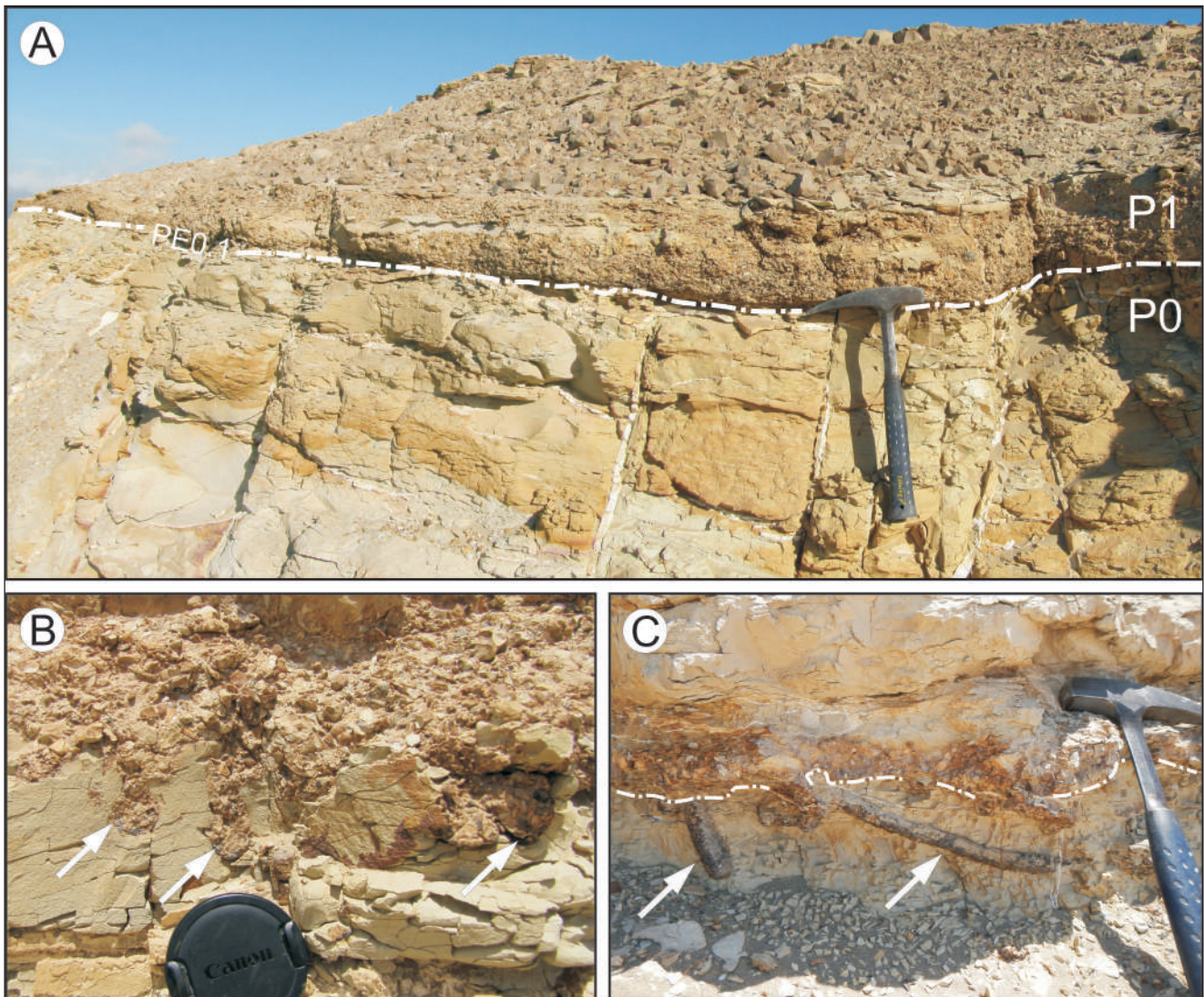
Fig. 3 - Details of the intraformational unconformities. A lens cap (6.5 cm in diameter) and a hammer (0.3 m long) are used for scale. A) Outcrop photograph of PE0.1 at Cerro las Tres Piramides ( 14^{\circ}35'15''\text{S} - 75^{\circ}38'38''\text{W} ). This surface is overlain by a lag comprised of rounded phosphate and igneous pebbles, reworked shells, and bones. B) The surface itself is generally sharp and undulating, bored and penetrated by robust Thalassinoides burrows (arrowed), which pipe dark phosphate pebbles of the P1 sequence for 0.3 m into the underlying P0 sequence. C) Detail of PE0.0 ( 14^{\circ}35'41''\text{S} - 75^{\circ}40'5''\text{W} ) showing inclined, smooth-walled Thalassinoides shafts weathering out in positive relief (arrowed) and passively filled with granular phosphorite infiltrated from the overlying pebble lag.
