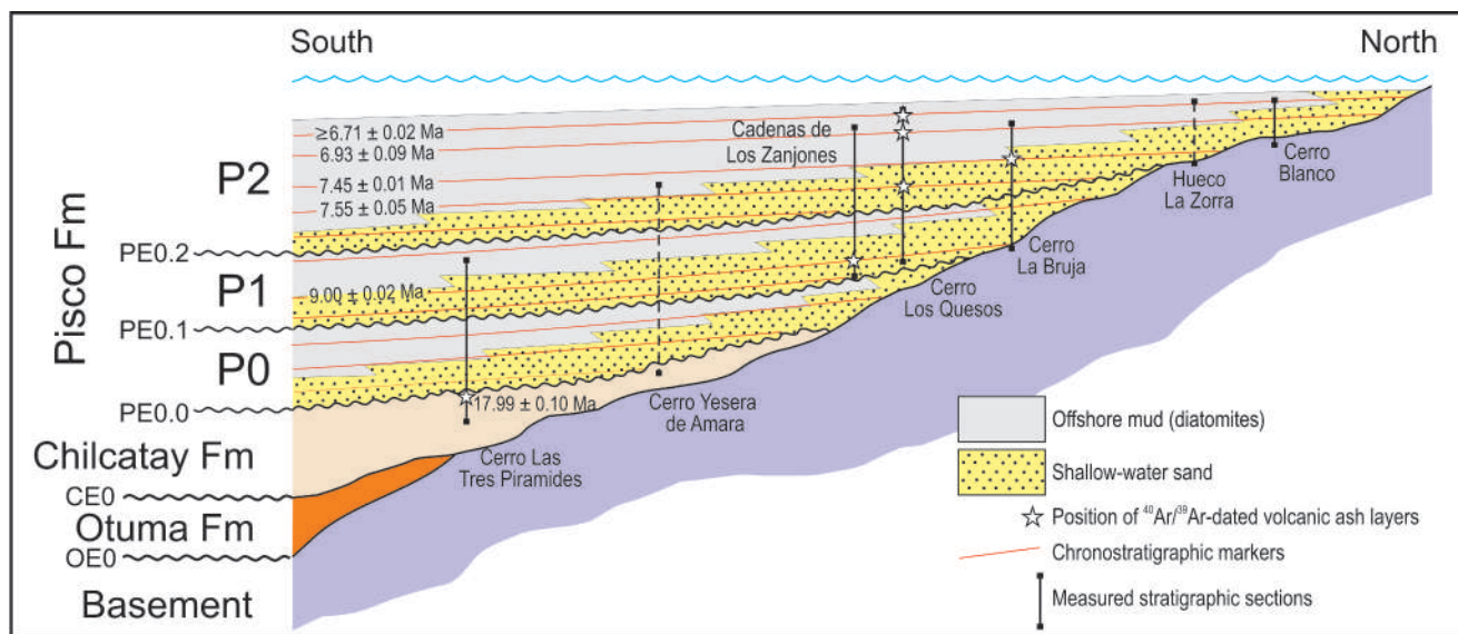
Fig. 6 - Schematic, dip-oriented stratigraphic diagram for the Pisco Formation (not in scale) showing the position of the stratigraphic sections on which the diagram is based (vertical black lines). These sections were supplemented by a cursory stratigraphic examination of two additional sites (vertical dashed lines). The Pisco Formation exhibits pronounced thinning to the northeast with component sequences onlapping onto the basal composite surface PE0 and arranged in a retrogradational pattern, progressively offset to the northeast. The marine erosion surfaces that bound Pisco sequences, namely PE0.0, PE0.1, and PE0.2, formed as a result of wave erosion in a transgressing shoreline following sea-level lowstand, and in consequence will be close to planar, and inclined slightly seaward. Red lines indicate chronostratigraphic markers (e.g., volcanic ash layers).
