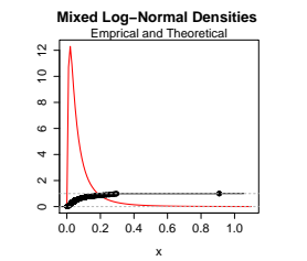
Fig. 44: Empirical and Theoretical Mixed Log-Normal Densities
