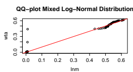
Fig. 65: QQ-plot of Mixed Log-Normal Distribution
