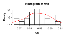
Fig. 8: Histogram of inter-arrival times of second part
