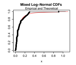
Fig. 45: Empirical and Theoretical Mixed Log-Normal CDF
