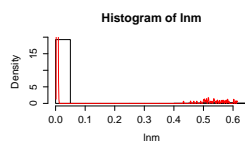
Fig. 64: Histogram of log-normal distribution
