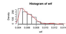
Fig. 7: Histogram of inter-arrival times of first part
