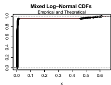
Fig. 56: Empirical and Theoretical Mixed Log-Normal CDF
