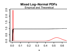
Fig. 66: Empirical and Theoretical Mixed Log-Normal Densities
