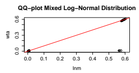
Fig. 9: QQ-plots of Mixed Log-Normal Distribution
