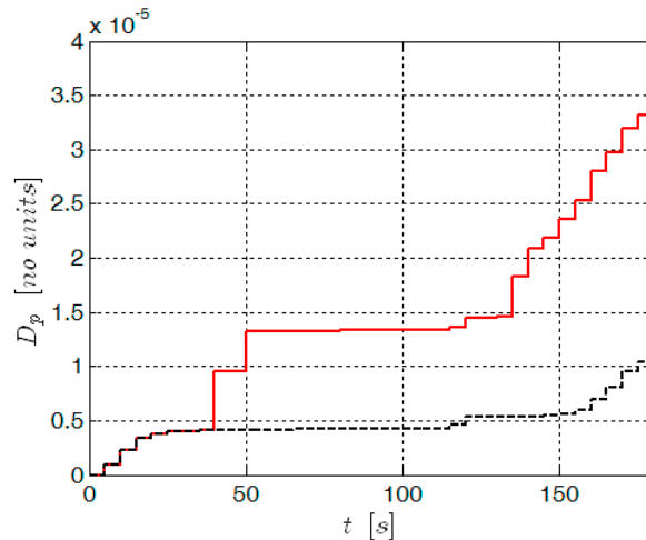
Fig. 10. Comparison between cumulative damage time histories obtained by proposed module for the two simulations. Red continuous line: non-stationary wind; black dashed line: stationary wind
