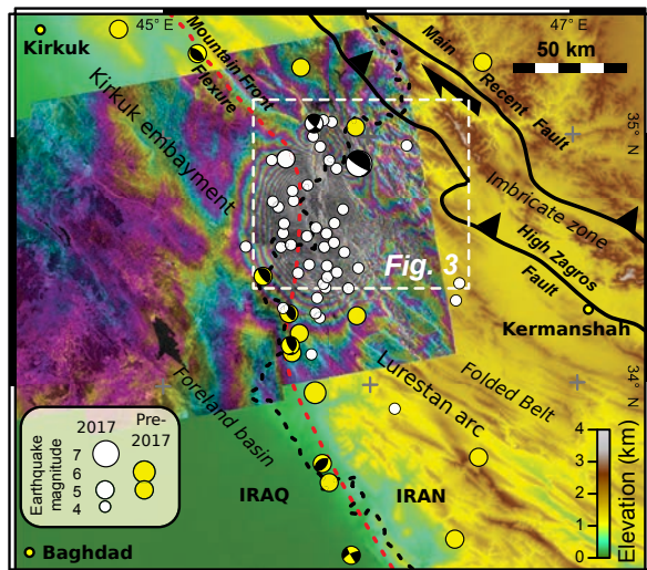
Figure 2. Elevation map (source: ESDIS) showing the main structural features of the Lurestan region and earthquake distribution (source: USGS, https://earthquake.usgs.gov/ ). M_w > 4 earthquakes of the November 2017 sequence are reported in white; pre-2017 M_w > 5 earthquakes are reported in yellow. The Sentinel 1 co-seismic interferogram (11 November, 15:00 UTC to 17 November 2017, 14:59 UTC; http://sarviews-hazards.alaska.edu/Event/34/ ; last access: 18 June 2018) is also shown as an overlay.
