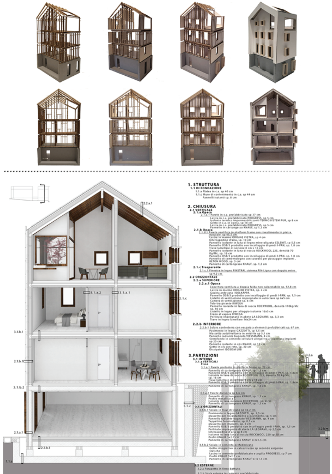
Figure 3: Strategies technological-constructive and detail section of new buildings.
