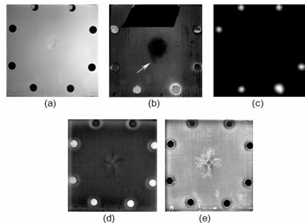
Figure 3. Laminate impacted at 22.5 J: (a) SWIRR result at 1650 nm, (b) Image subtraction between the reflectogram and the transmittogram acquired at 1650 nm, (c) Distance Transform (DT) applied on Fig. (b), (d) Correlation result, and (e) Kurtogram
