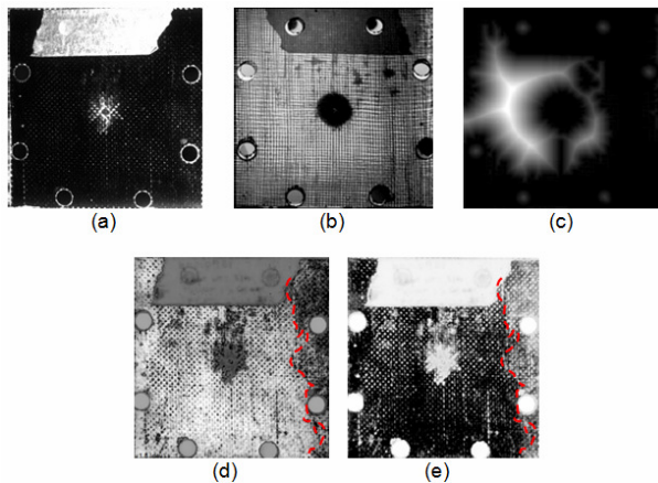
Figure 1. Laminate impacted at 7.5 J: (a) SWIRR result at 940 nm, (b) Image subtraction between the reflectogram and the transmittogram acquired at 940 nm, (c) Distance Transform (DT) applied on Fig. (b), (d) Correlation result, and (e) Kurtogram
