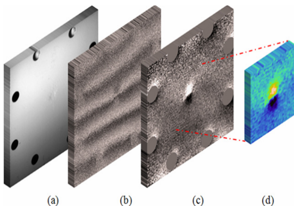
FIGURE 4. Laminate impacted at 22.5 J: (a) Visible image, (b) Phase image, (c) Phase image processed, and (d) Phase image detail in false colors centred on the impacted zone
