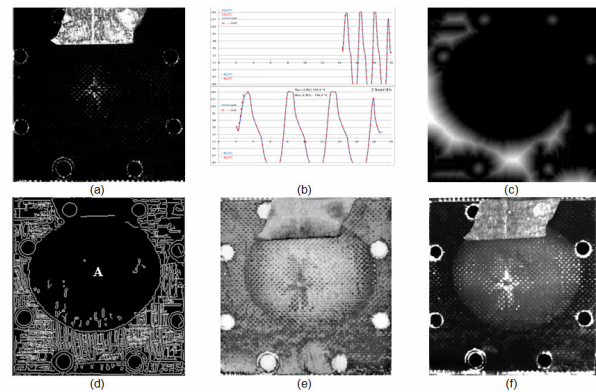
Figure 2. Laminate impacted at 15 J: (a) SWIRR result at 940 nm, (b) Graph inherent to the accelerated aging cycle, (c) Distance Transform (DT) applied on the image subtraction result, (d) Segmentation process after the image subtraction between the reflectogram and the transmittogram acquired at 940 nm, (e) Correlation result, and (f) Kurtogram
