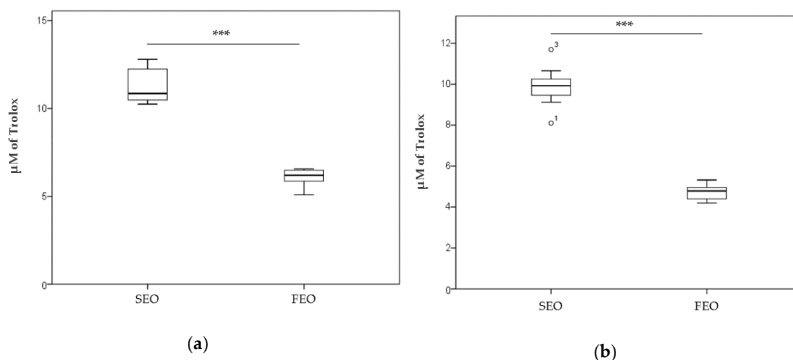
Figure 2. (a) Total antioxidant activity (TAA) measured in 2 mL of 2,2'-azinobis-(3-ethylbenzothiazoline-6-sulfonic acid) (ABTS) solution in the presence of 20 \mu\text{L} of SEO and FEO. The decrease in absorbance at 734 nm of ABTS solution is referred to a standard curve obtained by using known concentrations of Trolox. (b) Antioxidant activity versus DPPH radical was measured in 2 mL of DPPH solution in the presence of 50 \mu\text{L} of SEO and FEO. The decrease in absorbance at 517 nm is referred to a standard curve obtained using known concentrations of Trolox ( \mu\text{M} ). *** p < 0.001 . o^1 , o^3 : outliers values.
