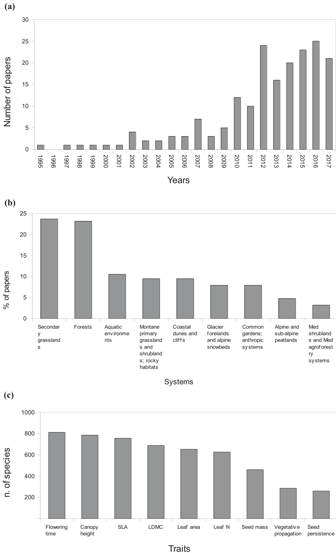
Figure 1. Italian studies on functional traits in relation to environmental variables/gradients: (a) temporal trend in the number of papers published per year; (b) distribution of the collected papers regarding studied ecosystems; (c) number of vascular plant species accounted for the most frequently investigated functional traits.
