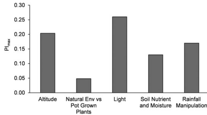
Figure 3. Maximum values of plasticity index (PI, sensu Valladares et al. 2000) of Specific Leaf Area for the endemic Sesleria nitida in different environments or along gradients (altitude, Gratani et al. 2014; natural environment vs. pot grown plants, Puglielli et al. 2015b; Light, Puglielli et al. 2015a; soil nutrient and moisture, Wellstein et al. 2013; rainfall manipulation, Wellstein et al. 2017).
