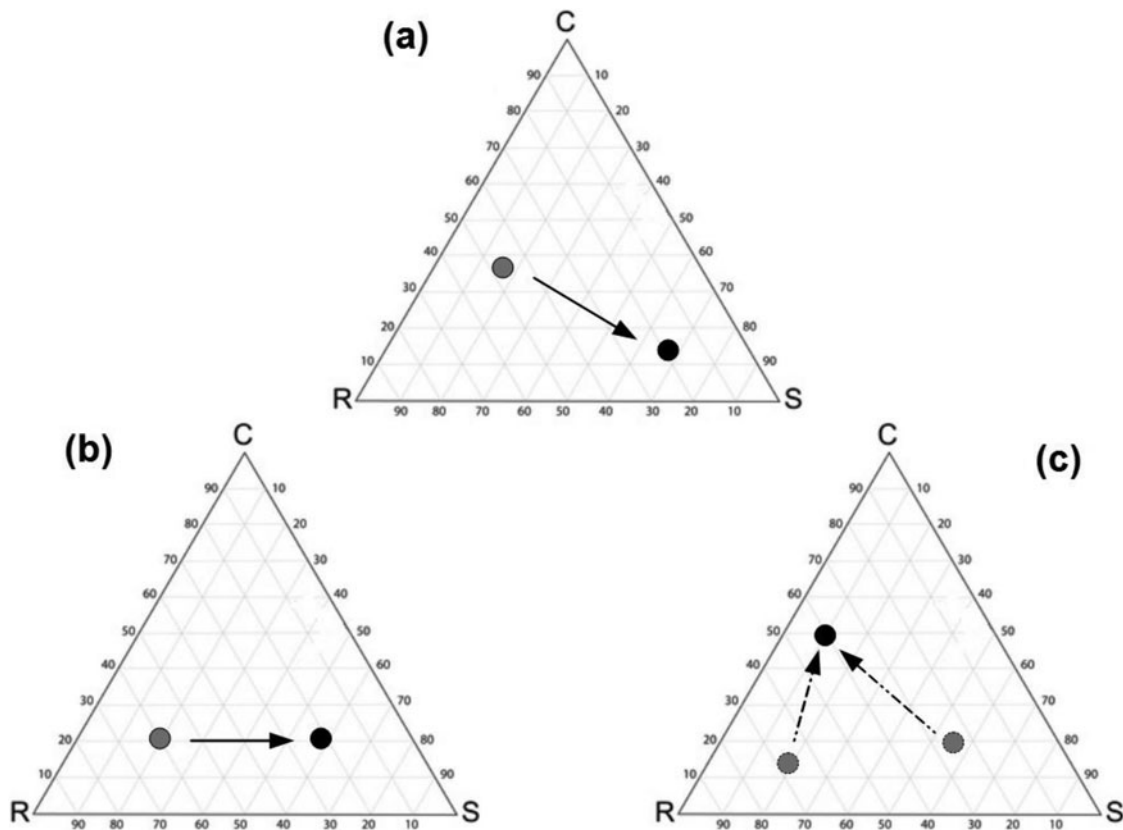
Figure 2. CSR triangles synthesizing general mean strategies and shifts of vegetation along gradients of (a) increasing elevation (based on Caccianiga et al. 2006; Pierce et al. 2007a, 2007b; Gentili et al. 2013), (b) primary successions, including glacier forelands and coastal dunes (based on Caccianiga et al. 2006; Gobbi et al. 2010; Ciccarelli 2015), and (c) grazing abandonment (based on Pierce et al. 2007a; Cerabolini et al. 2010a).
