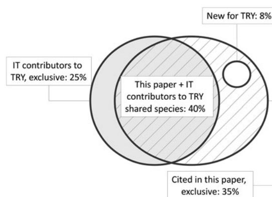
Figure 4. Gathered information on plant traits of Italian populations deriving from our review ( Supplementary Information Appendix 2 ) and the Italian contributors to TRY, for an overall total of 1418 taxa, almost the 20% of the entire Italian vascular flora (Bartolucci et al. 2018). Traits measurements of about 900 species (65% of the 1418 taxa) are already shared in TRY database (i.e. species found both in the reviewed papers and in the Italian datasets contributing to TRY, or species found only in the Italian datasets contributing to TRY), while trait values for 502 species (35% of the 1418 taxa) recorded by this review are not available in TRY; among these latter, 113 species (8% of the 1418 taxa) are totally missing in TRY.
