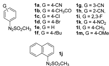
Chart 1. Arylazo Sulfones Used in the Present Study
