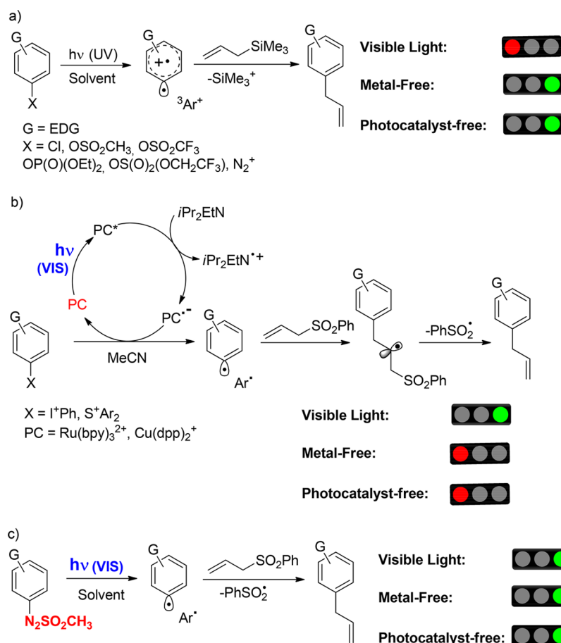
Scheme 1. Photochemical/Photocatalyzed Synthesis of Allylarenes
