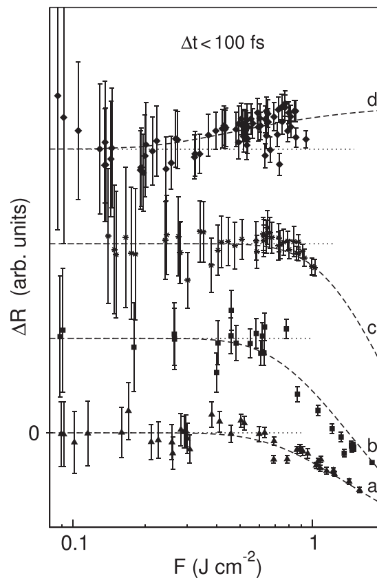
FIG. 3. FEL-driven ultrafast ( \approx 100\ \text{fs} ) changes of the EUV reflectivity of Ti (for the same photon energies of Fig. 2). Data shown in the plot are proportional to the variation of reflectivity and are vertically shifted to facilitate the readability. Dotted horizontal lines indicate the \Delta R = 0 level. The dashed curves are guides to the eye. Error bars reflect a 1-\sigma confidence interval.
