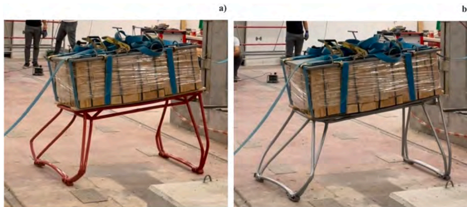
Fig. 17. Impact test performed with a brick stack of 450 kg: a) impact moment on V prototype; b) impact moment on S prototype.
