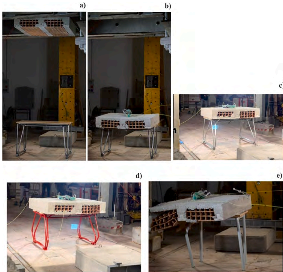
Fig. 18. Impact test performed with a floor portion of 300 kg: a) test setup prior to release; b) impact moment on S prototype; c) after the impact moment on S prototype; d) after the impact moment on V prototype; e) after the impact moment on traditional desk.
