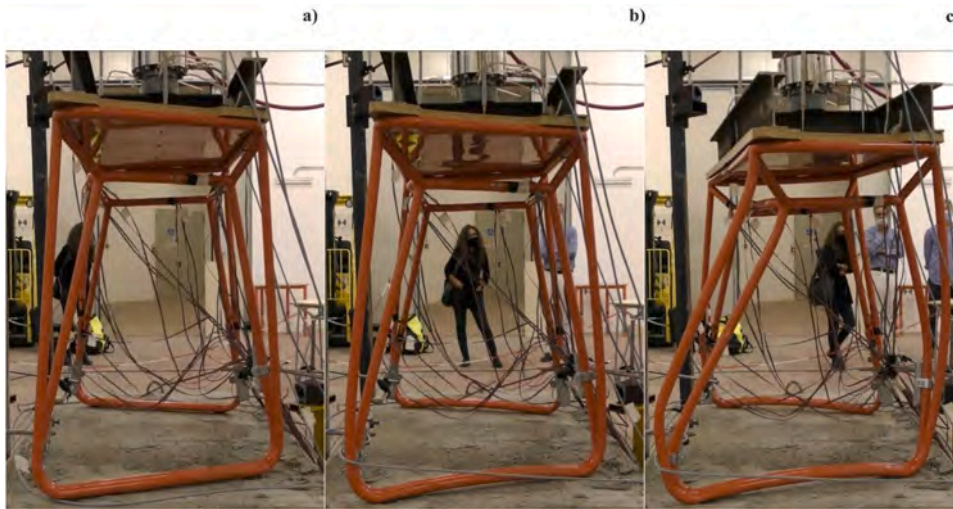
Fig. 12. From left to right, the start of the test, the incipient of buckling, and the final shape of the specimen, respectively.
