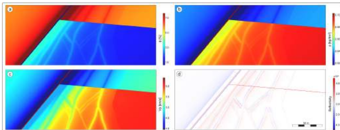
Fig. 11. a) Porosity ( \phi ), b) Bulk density ( \rho ), c) P-wave velocity ( V_p ), and d) reflectivity of the GM2 base model, assuming an E/l ratio = 0.005.
