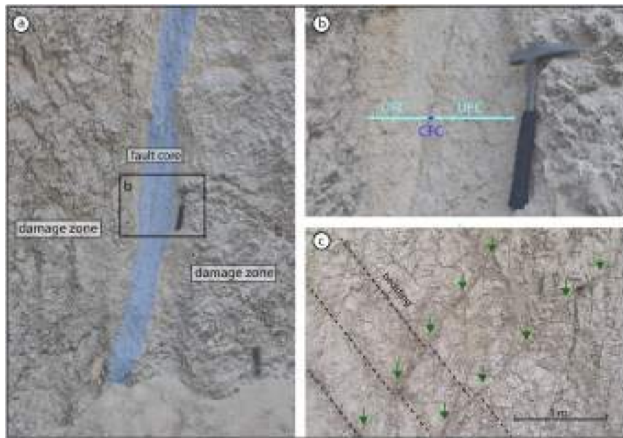
Fig. 7. Detail of the inner architecture of subsidiary faults on the eastern wall. a) 2nd order fault zone and associated close-up in (b), b) uncemented (UFC) and cemented (CFC) fault rocks, c) two 3rd order faults highlighted by green arrows, including pods of fault breccia and clearly offsetting bedding. (For interpretation of the references to colour in this figure legend, the reader is referred to the Web version of this article.)
