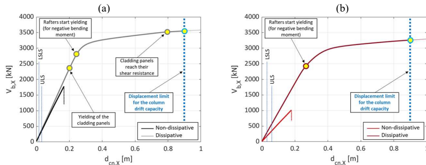
Fig. 8. Pushover results for the transverse direction: (a) model with panels; (b) bare frame
