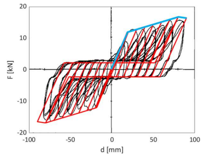
Fig. 6. Cladding panels: experimental vs numerical cyclic response.
