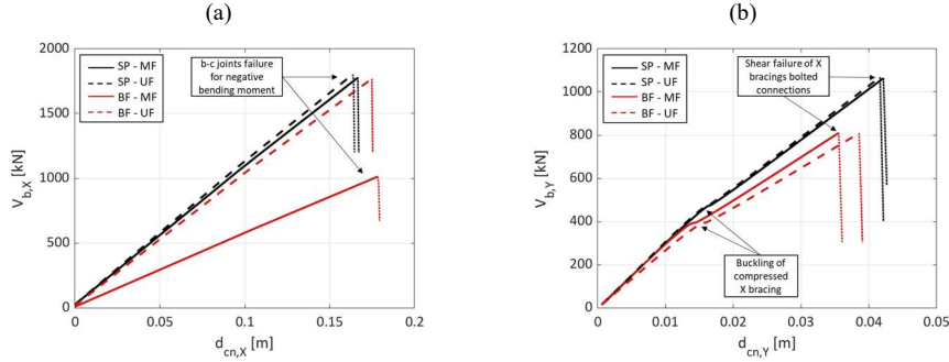
Fig. 7. Pushover results for the “non-dissipative” structure: (a) transverse (X) direction; (b) longitudinal (Y) directions.
