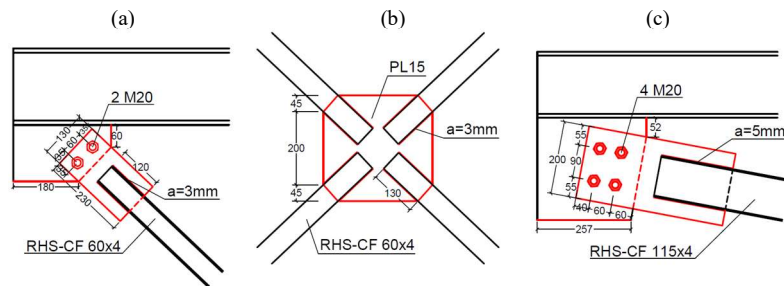
Fig. 2. End (a) and central (b) connections of the X-bracing system; brace connections for the single-diagonal bracing system (c).
