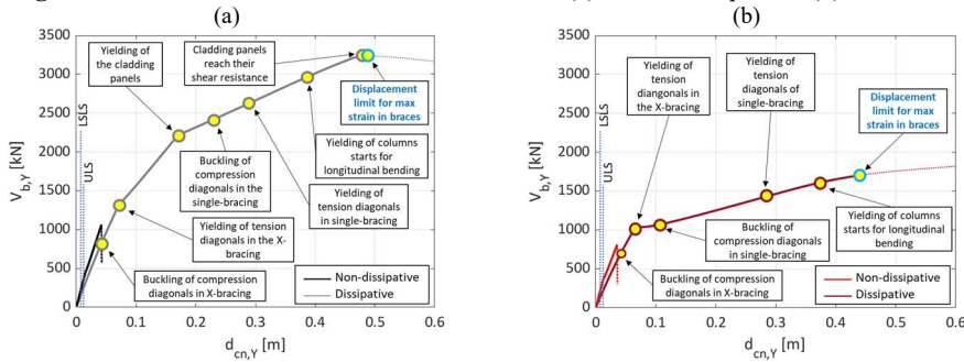
Fig. 9. Pushover results for the longitudinal direction: (a) model with panels; (b) bare frame
