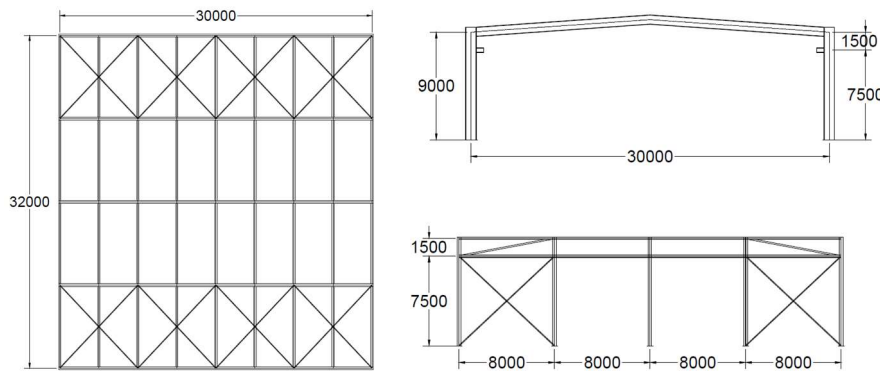
Fig. 1. Global geometry of the case study.
