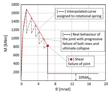
Fig. 5. Moment vs. rotation for beam-column joints.
