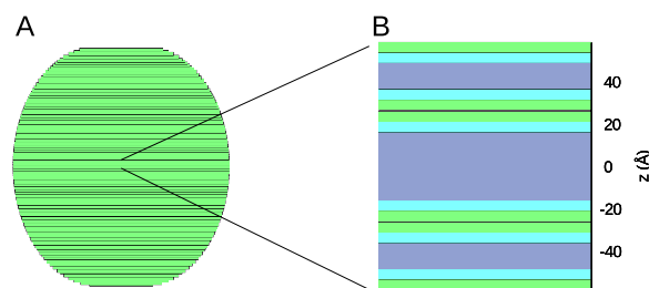
Fig. 11. Panel A: Representation of a LNP with external and internal dimensions corresponding to the medians of the distributions derived from the analysis of SAXS data at C_{\text{LNP}} = 80.0 \text{ g/L} and 20 °C. (Fig. 10, R_M = 1520 \text{ Å} , H = 3390 \text{ Å} , 2(t_0 + t_1 + t_2 + \Delta t/2) = 39 \text{ Å} ). Panel B: three platelets in the core, with layers schematically representing hydrated P80 polar heads (green), mixed P80 hydrophobic chains (cyan) embedded in amorphous CP (cyan) and lamellar CP (blue). The thicknesses of the blue layers were sampled from the derived p_i(t) distribution.
