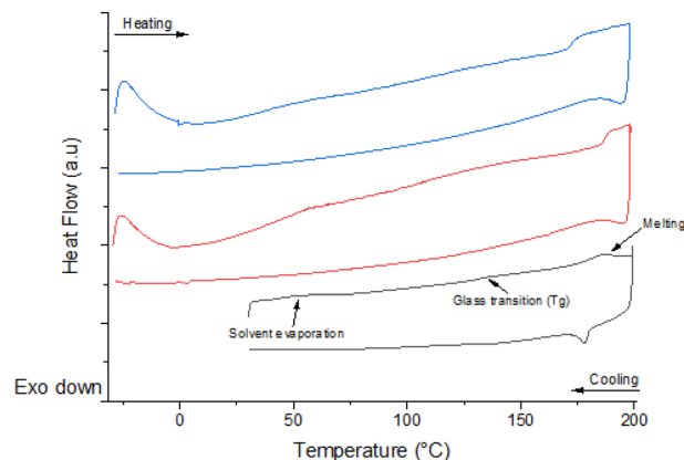
Fig. 5 DSC traces of EC1a-P4 (blue line), EC-P4 (red line) and EC0 (black line) (from ref. 32) obtained at a heating rate of 5\text{ °C min}^{-1} .
