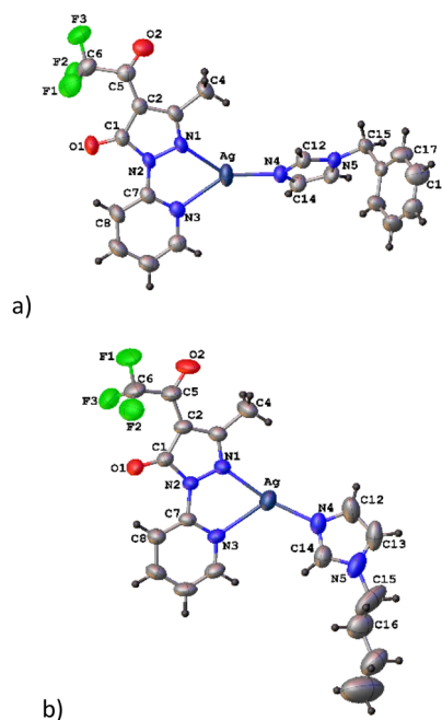
Fig. 2 Molecular structure of (a) [Ag(Q py,CF3 )(Bn-Im)], 1, and (b) [Ag(Q py,CF3 )(Bu-Im)], 2, with the atomic labelling scheme.
