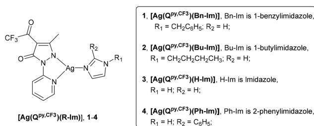
Fig. 1 Structure of complexes [Ag(Q^{Py,CF_3})(R-Im)] , 1–4.
