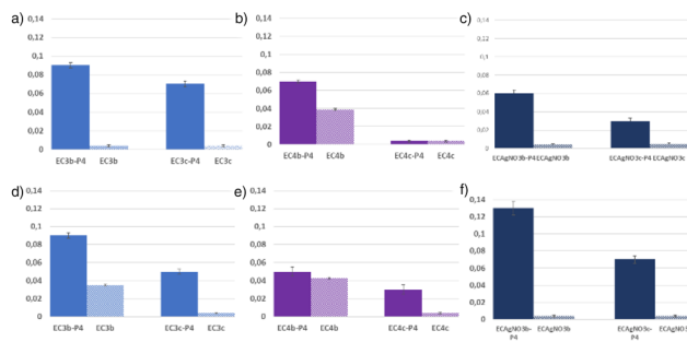
Fig. 16 Ag(I) migration values in milligrams per volume of EC3b,c-P4, EC3b,c, EC4b,c-P4, EC4b,c, ECAGNO 3 b,c-P4 and ECAGNO 3 b,c films in simulant B at (a), (b) and (c) 2 h and 70 °C and (d), (e) and (f) 10 days at 40 °C.
