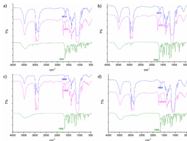
Fig. 10 FT-IR spectra of (a) EC1a, EC1a-P4 and complex 1 ; (b) EC2a, EC2a-P4 and complex 2 ; (c) EC3a, EC3a-P4 and complex 3 ; and (d) EC4a, EC4a-P4 and complex 4 . Non-plasticized and plasticized films: blue and pink lines and complexes 1 – 4 : green line.
