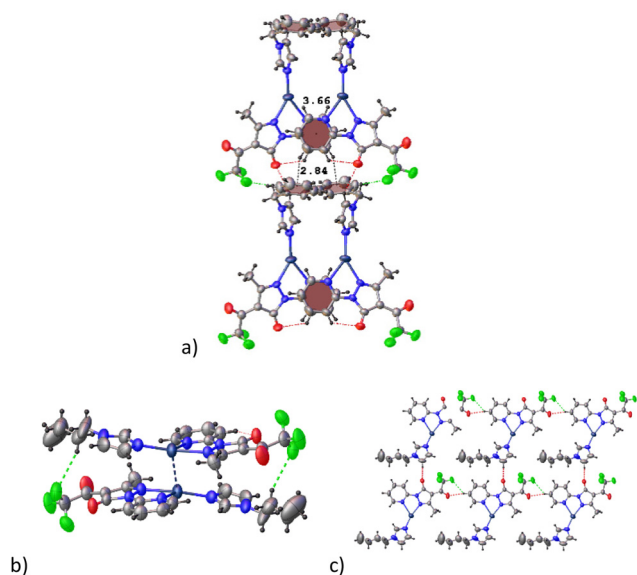
Fig. 3 Crystal packing view of (a) complex 1 (down the a direction) showing \pi – \pi – \pi C–H– \pi , C–H–O and C–H–F interactions, and (b) complex 2 along the b direction and in the ac plane.
