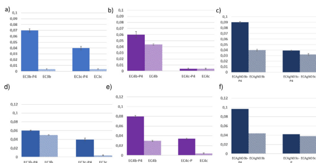
Fig. 15 Ag(I) migration values in milligrams per volume of EC3b,c-P4, EC3b,c, EC4b,c-P4, EC4b,c, ECAGNO 3 b,c-P4 and ECAGNO 3 b,c films in simulant A at (a), (b) and (c) 2 h and 70 °C and (d), (e) and (f) 10 days at 40 °C.
