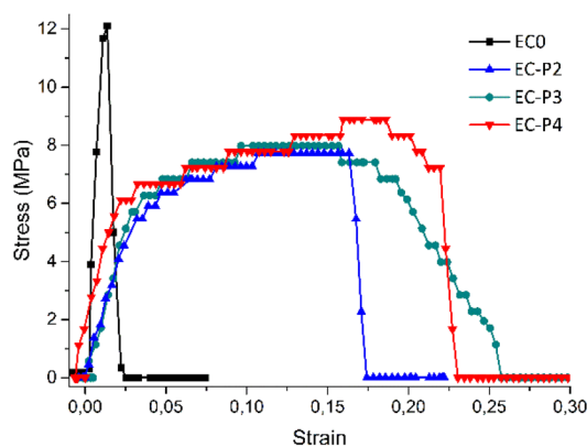
Fig. 4 Comparison of stress vs. strain plots between EC films and EC-P films.
