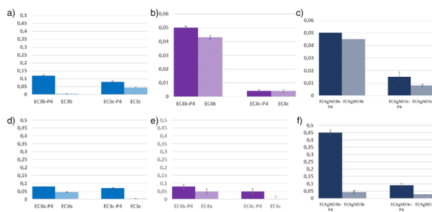
Fig. 17 Ag(I) migration values in milligrams per volume of EC3b,c-P4, EC3b,c, EC4b,c-P4, EC4b,c, ECAGNO 3 b,c-P4 and ECAGNO 3 b,c films in simulant C at (a), (b) and (c) 2 h and 70 °C and (d), (e) and (f) 10 days at 40 °C.
