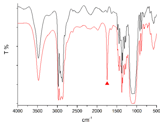
Fig. 9 FT-IR spectra of EC0 (black line) and EC-P4 (red line).
