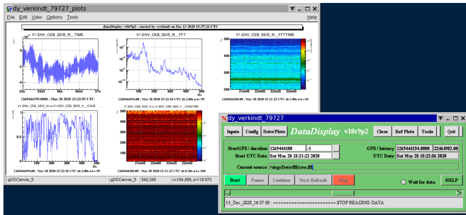
Figure 10. Example of the plots produced by the dataDisplay (left) and main panel of the dataDisplay graphical user interface (right).
