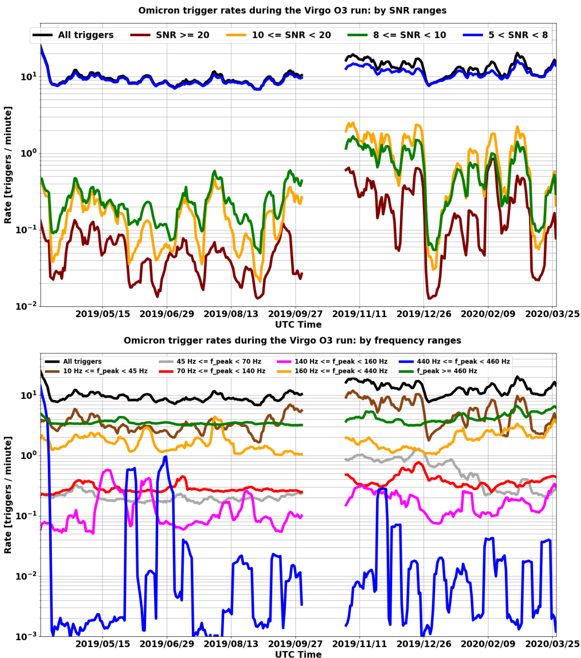
Figure 26. Glitch rates (weekly moving average) using Omicron triggers during the O3 run for Virgo—the gap in between O3a and O3b corresponds to the 1-month commissioning break. The top plot breaks the glitch rate into SNR ranges, while the bottom one categorizes it in terms of frequency ranges for the glitch peak frequency. The choice of the frequency bands has been mainly driven by the need to isolate some frequencies: 50 Hz (mains fundamental power in Europe), 150 Hz (second harmonics of the mains) and the range around 450 Hz (another harmonics of the mains, plus the range in which the frequencies of the suspension wire violin modes are located).
