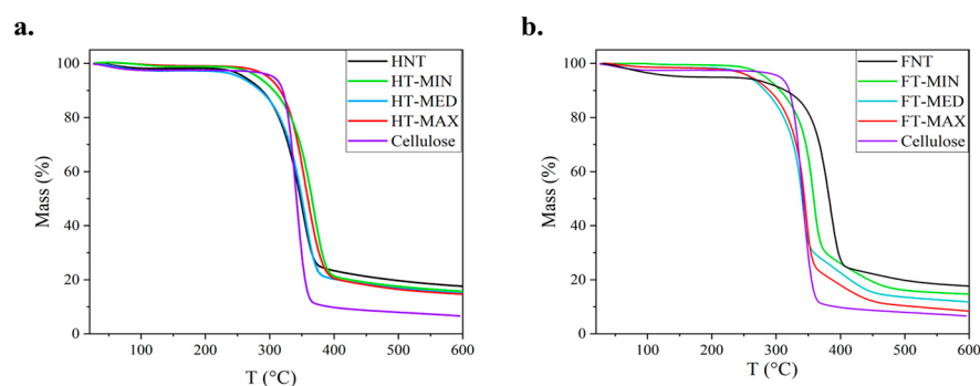
Figure 5. Thermogravimetric analysis (TGA) for (a) treated and untreated hemp samples and (b) treated and untreated flax samples, in both cases, compared to reference cellulose.
