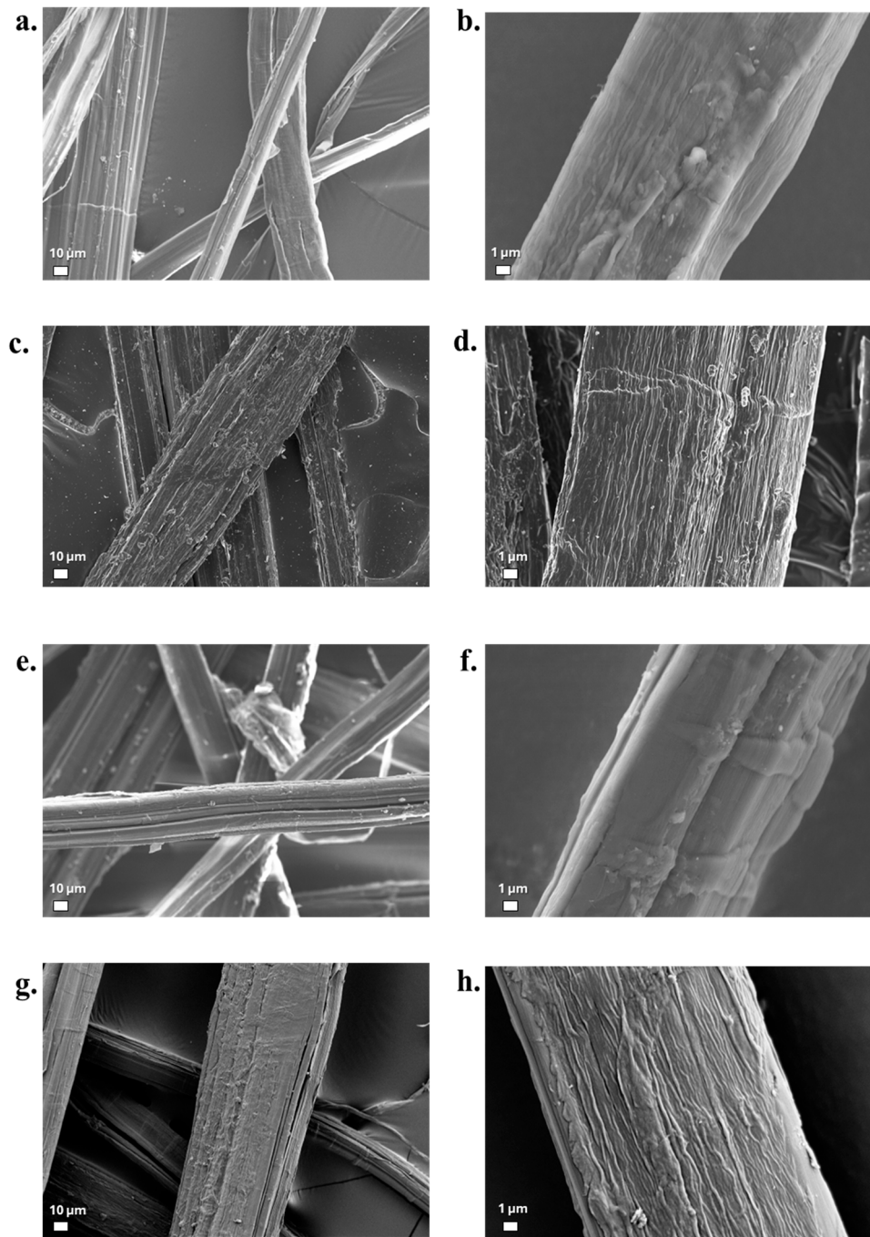
Figure 10. SEM morphological observations for different untreated and treated hemp fibres: (a,b) HNT, (c,d) HT-MIN, (e,f) HT-MED, (g,h) HT-MAX.
