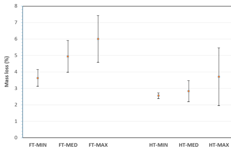
Figure 4. Mass loss (%) for treated fibres with selected combinations.
