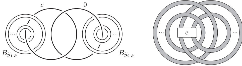
FIGURE 1. Ribbon fillability of \tilde{p}|\partial .
