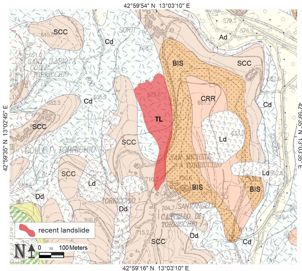
Figure 4 - Geological map of the Torricchio Landslide (TL): Cd-Colluvial deposits, Ad-Alluvial deposit, Dd-Debris deposit, CRR-Marne con Cerrognà (marls), BIS-Bisciaro (marls and marly limestones), SCC-Scaglia cinerea (marly limestones and marls, with intercalations of argillites); (base map from the open data of the Marche Region geological database, https://www.regione.marche.it/Regione-Utile/Paesaggio-Territorio-Urbanistica/Cartografia/Repertorio/Cartageologicaregionale10000 , modified).
