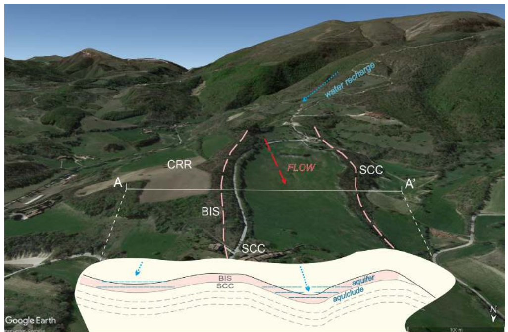
Figure 20 - Interpretative 3-D sketch of the hydrogeological structures that favour the accumulation and occasional overflow of water triggering flow landslides. CRR (Marne con Cerrognna), BIS (Bisciaro) and SCC (Scaglia cinerea) represent the bedrock formations; A-A' schematic cross section (base image from Google Earth, 2024).
