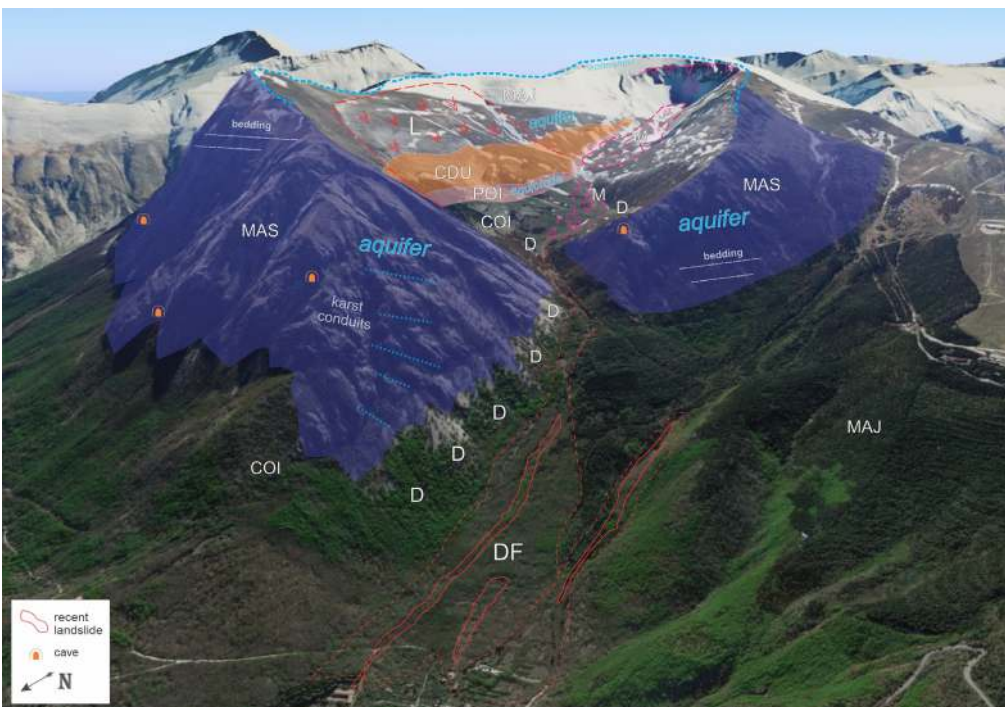
Figure 18 - Geological and geomorphological sketch interpreting the dynamics of processes in the VU area (Monte Bove relief). MAS-Calcare massiccio, COI-Corniola, POD-Marne a Posidonia, CDU- Calcari Diasprini U.M., MAJ-Maiolica, M- relict glacial deposits, D-coarse Debris and blocks, DF-debris flow area, in continuous red line the recent ones (base image from Google Earth, 2024).
