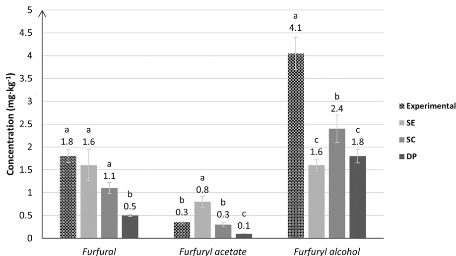
Fig. 1. Average values of furfural, furfuryl acetate and furfuryl alcohol found in the experimental biscuits baked under optimal conditions (at 175 °C static for 22 min and ventilate for 20 min) and in commercial Shortbreads with Eggs (SE), Shortbreads with Chocolate chips (SC) and Dry Petit (DP) biscuit types. Different letters in the same compounds indicate significant differences among samples at p < 0.05 level.
