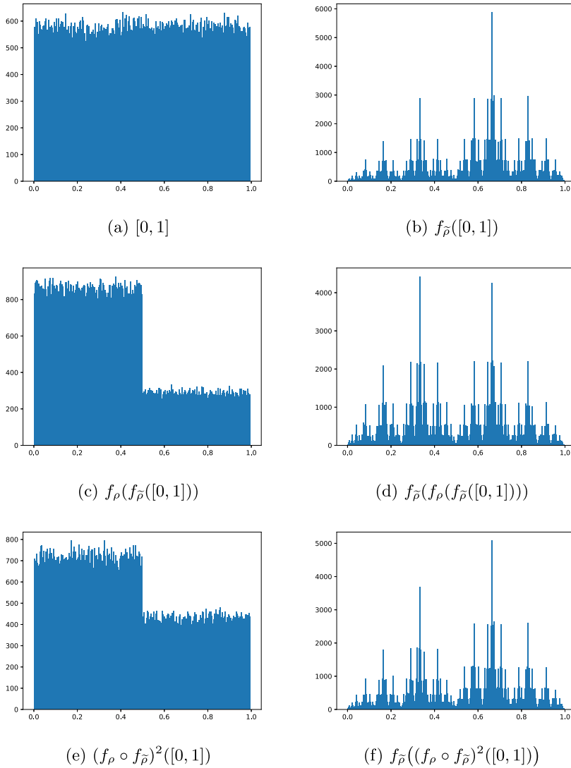
FIGURE 5. Numerical results on the first iterates of f_{\rho} \circ f_{\tilde{\rho}} . The graphs show how many, out of approximately 150,000 randomly selected points from [0, 1] , occupy the subintervals of length 2^{-8} at each iterate.
