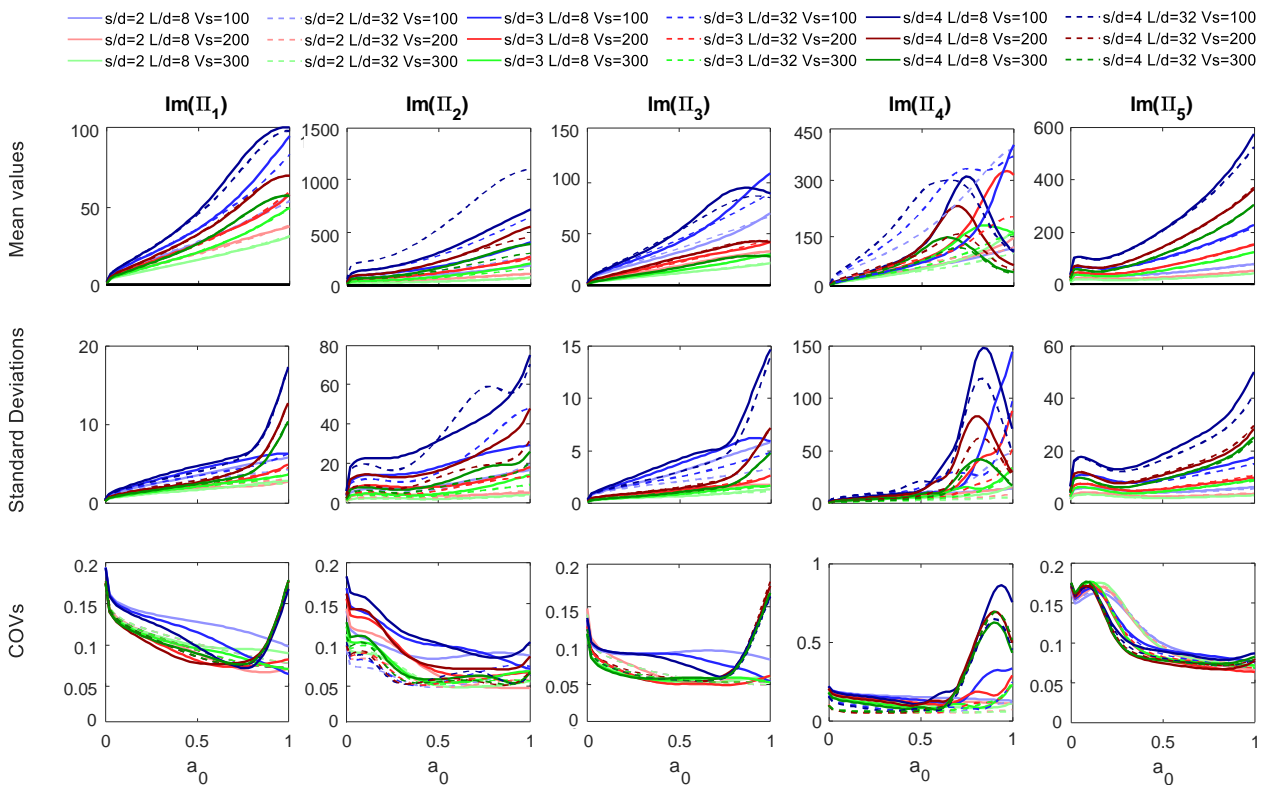
Figure 11. Frequency dependent mean values, standard deviations and COVs of imaginary parts of non-dimensional impedances of 2x2 foundations
