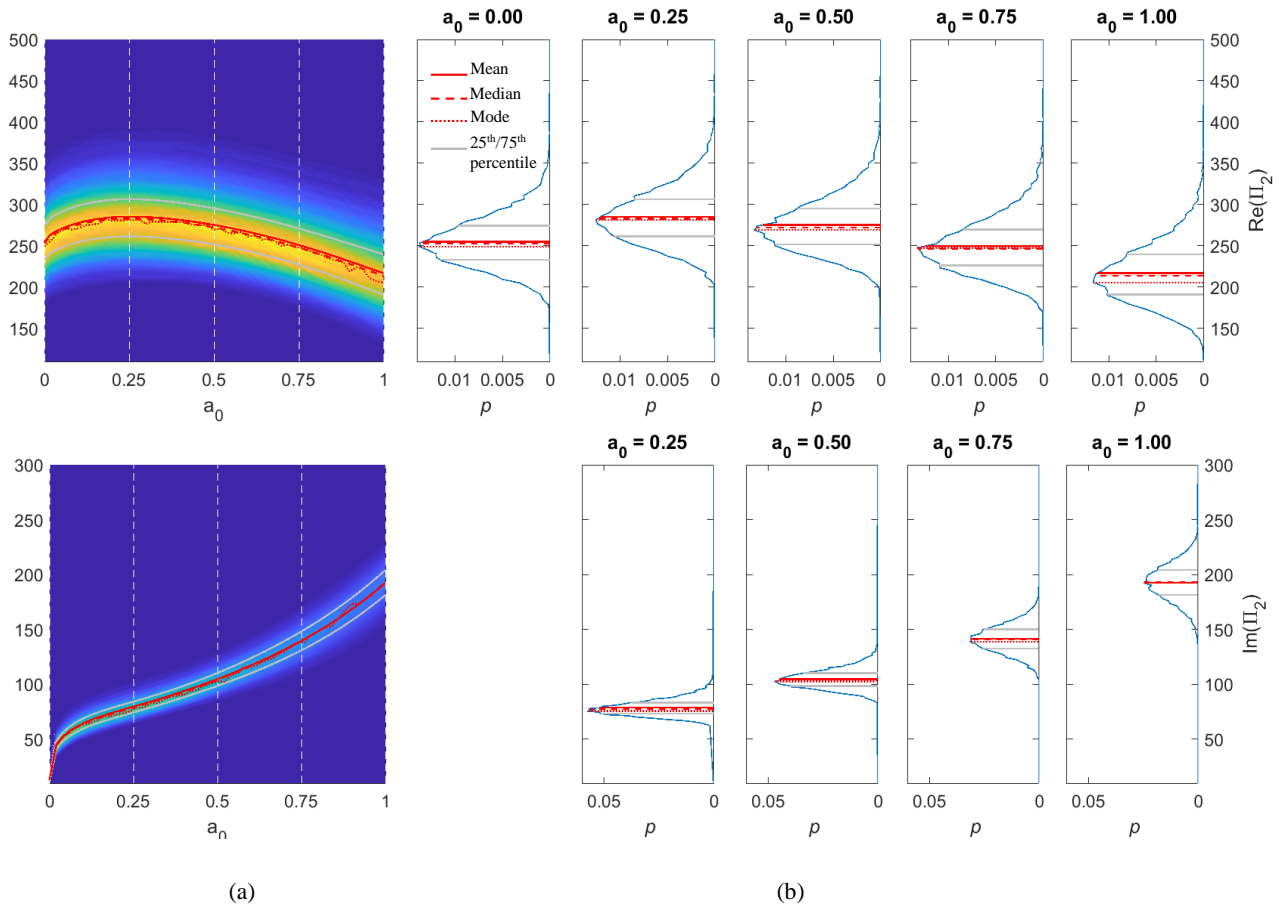
Figure 7. (a) Variability of \Pi_2 (real and imaginary parts) and (b) distributions of values at selected frequencies Case 2x2, s/d = 2 , L/d = 8 , V_s = 100 m/s
