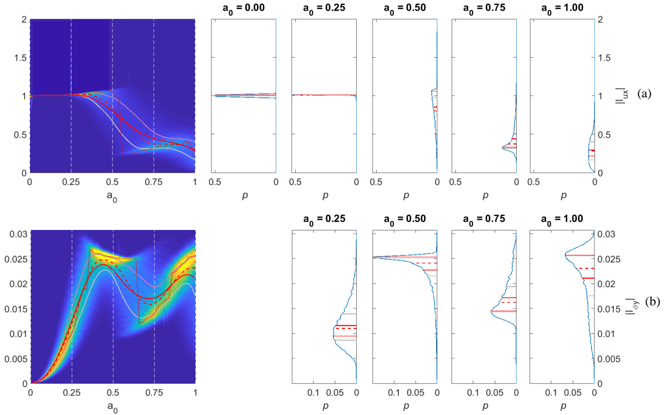
Figure 16. Variability of (a) I_U and (b) I_\Phi for 3x3 foundation, s/d = 4 , L/d = 32 , V_s = 100 m/s
