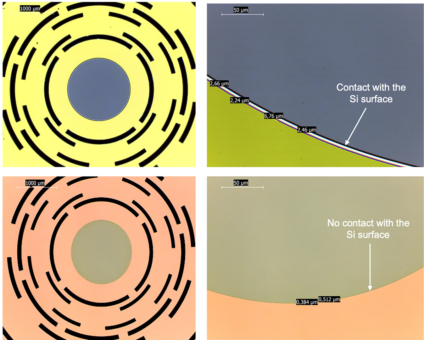
FIG. 6. Round-shaped Si 3 N 4 membrane surrounded by the on-chip filter and a detailed view of the membrane's edge. (Top) Case of Si 3 N 4 deposited on a LPCVD TEOS oxide sacrificial layer where the membrane is stitched on the Si substrate. (Bottom) Case of Si 3 N 4 deposited on a thermally grown oxide without membrane's stitching to the substrate.
