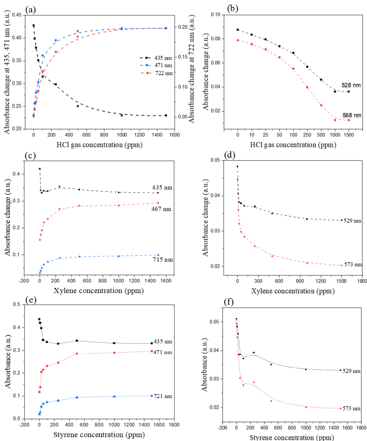
Figure 9. Linearity between absorbance change along with HCl gas concentration in UV-Vis absorption spectrum of PPc film interacting with (a,b) HCl vapor (10 ppm to 1500 ppm); (c,d) m-xylene vapor (10 ppm to 1500 ppm); (e,f) styrene vapor (10 ppm to 1500 ppm).
