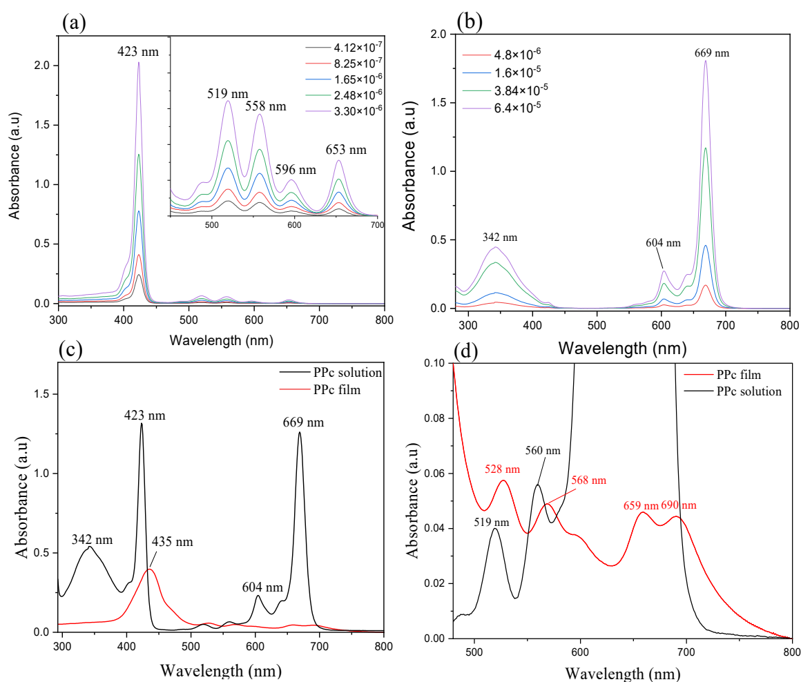
Figure 3. Absorption spectra of (a) THPP in DMF solution ( 4.1 \times 10^{-7} mol L -1 to 3.3 \times 10^{-6} mol L -1 ), (b) ZnPc in DMF solution ( 4.8 \times 10^{-6} mol L -1 to 6.4 \times 10^{-5} mol L -1 ), (c) PPc blend before and after film formation, (d) magnified spectra of the PPc blend in the range 500–800 nm.
