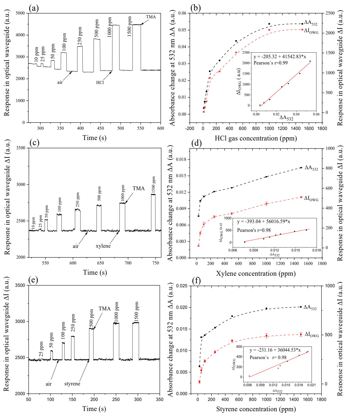
Figure 6. Planar optical waveguide response results along with time (a,c,e) HCl, m-xylene, and styrene exposures (10–1500 ppm; (b,d,f) correlation of the planar optical waveguide response and absorbance change at 532 nm as a function of gas concentration.
